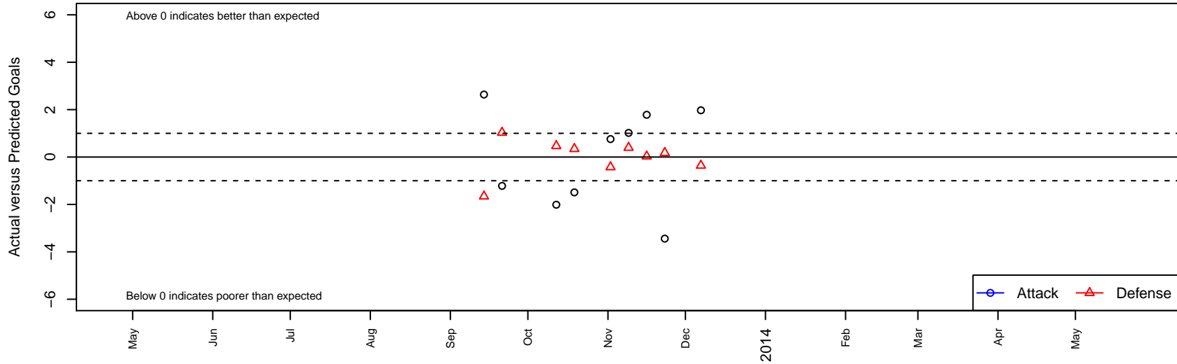
FSC Chickadees G01 Dots are actual minus expected GF (blue circles) and GA (red triangles). Blue line is smoothed change in attack strength. Red is smoothed change in defense strength.
